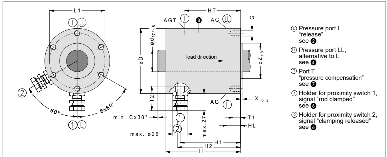
Fig. 1: Dimensions Safety Lock KRG
